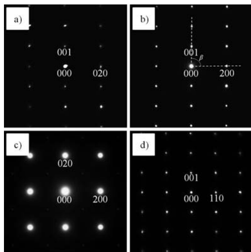
Figure 2. a) [100], b) [010], c) [001], and d) [-110] zone-axis selected-area electron diffraction patterns obtained for \text{BiFe}_{0.30}\text{Co}_{0.70}\text{O}_3 at 298 K. The electron diffraction spots are indexed on the cubic perovskite structure. The monoclinic angle \beta can be estimated to be approximately 91.4^\circ in the reciprocal lattice space. The space group is deduced to be Cm from the analysis of various ED patterns. The unit cell is \sqrt{2}a \times \sqrt{2}a \times a , where a represents the lattice parameter of the cubic perovskite structure.
