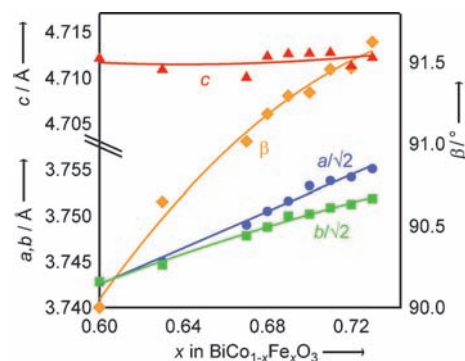
Figure 3. The composition dependence of the lattice parameters of monoclinic \text{BiCo}_{1-x}\text{Fe}_x\text{O}_3 ( 0.60 \leq x \leq 0.73 ).
